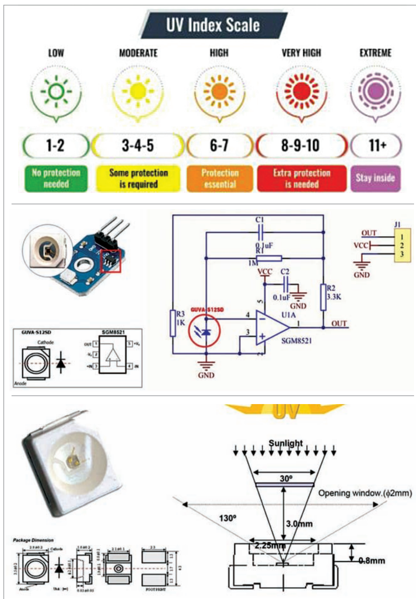
Fig. 4: The internal circuit diagram, working, and characteristics of the UV sensor
