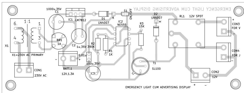
Fig. 4: Component layout for the PCB
