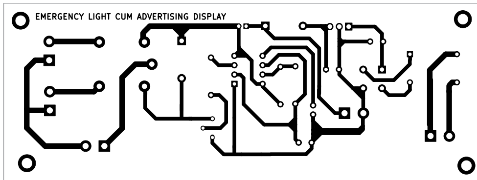
Fig. 3: Actual-size PCB layout of the circuit
