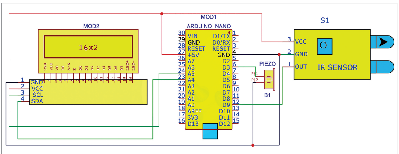
Fig. 2: Circuit diagram
