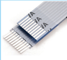
Open end Type for direct soldering
