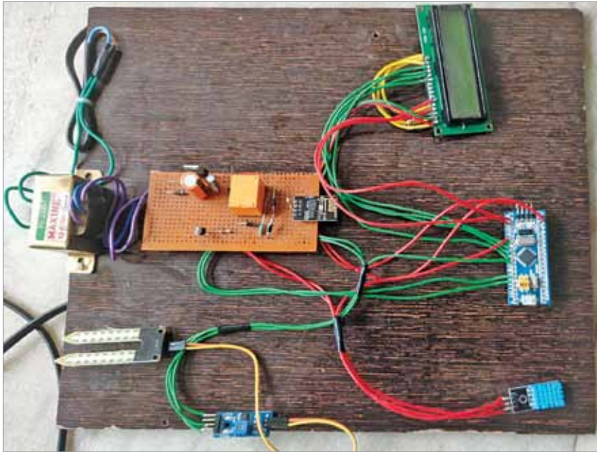
Fig. 17: The authors' prototype
