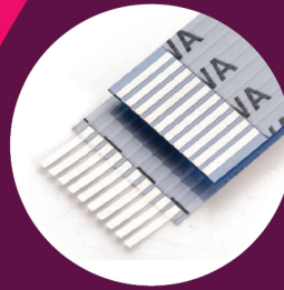
Open end Type for direct soldering
