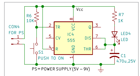
Fig. 1: Correct circuit for experiment 2
