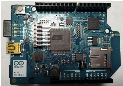
Fig. 5: Wireless shield attached to Arduino Uno
