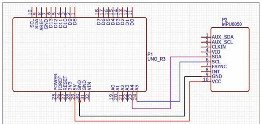
Fig. 2: Circuit diagram
