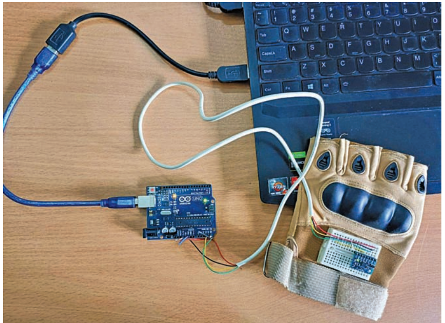
Fig. 1: Author's prototype
