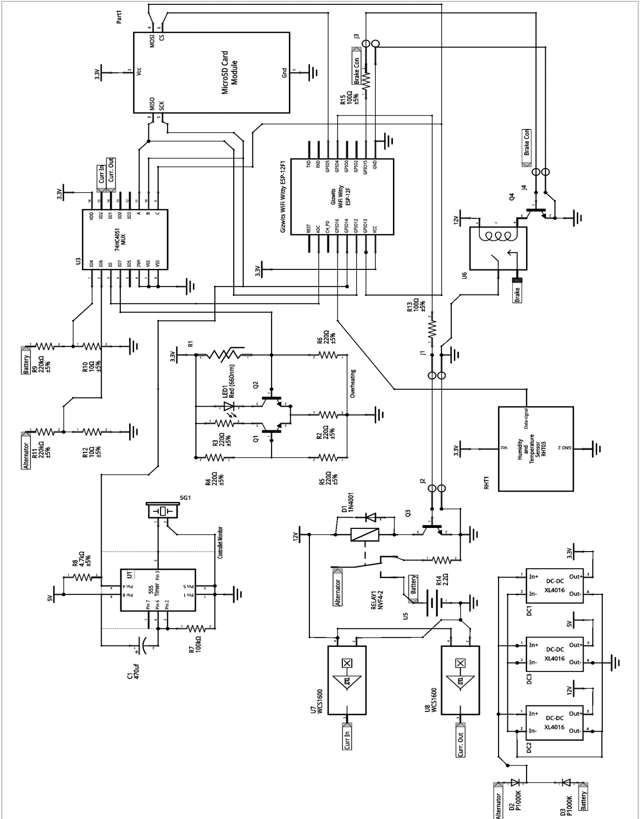
Charge controller circuit with safety features to detect and prevent serious problems
