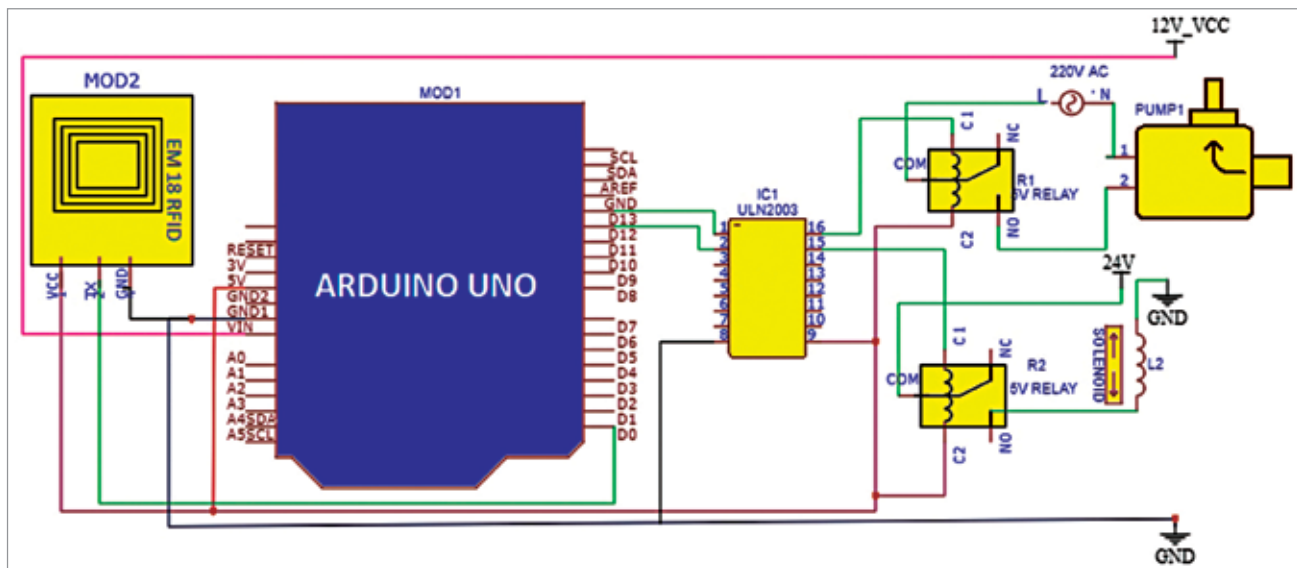
Fig. 5: Circuit diagram
