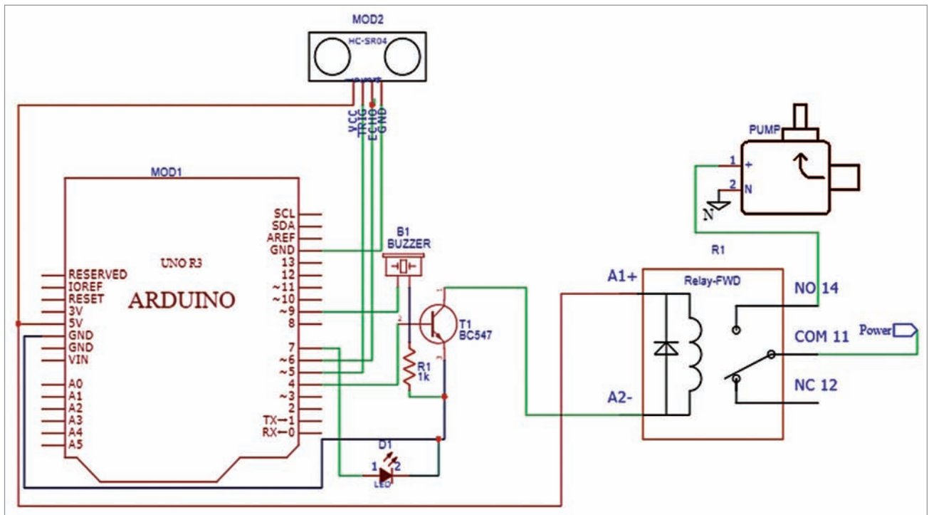
Fig. 2: Circuit diagram
