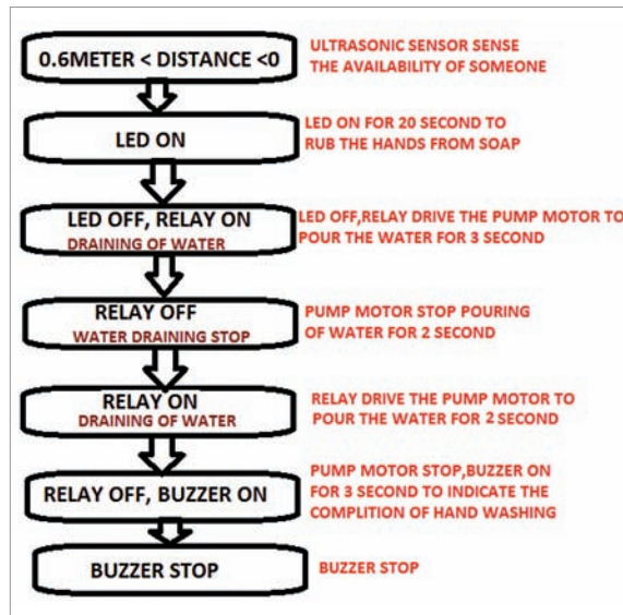
Fig. 1: Flow chart of the water dispenser
