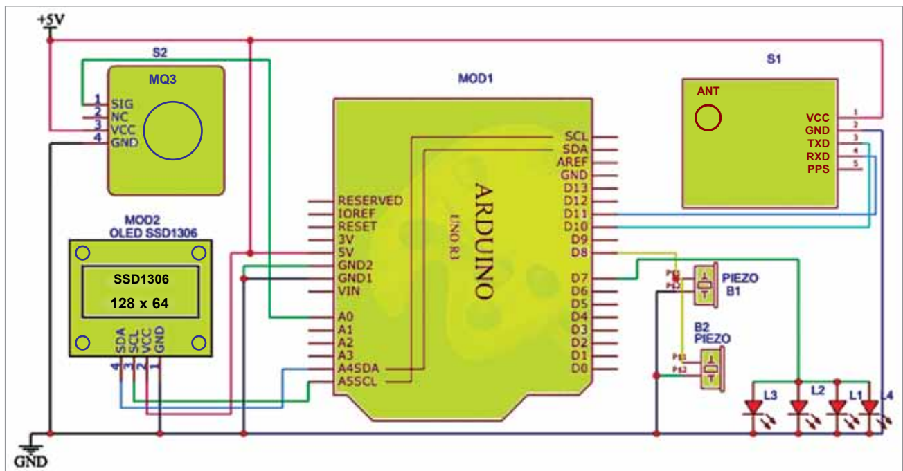
Fig. 2: Circuit diagram
