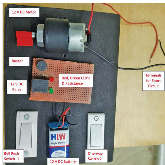
Fig. 3: Author's prototype of protection circuit
