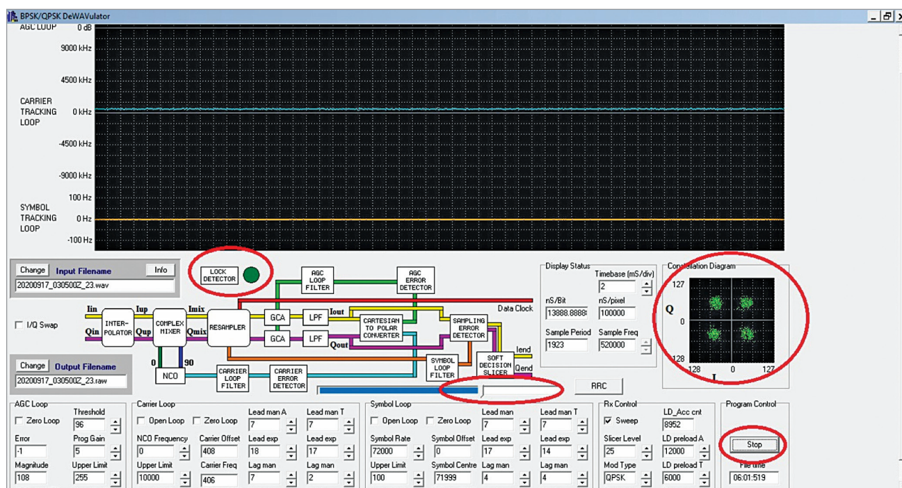
Fig. 8(b): LRPTX demodulation in progress (Note the fine dots in the constellation diagram)
