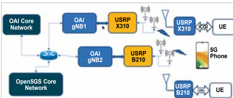
Fig. 1: Lab system: connection model
