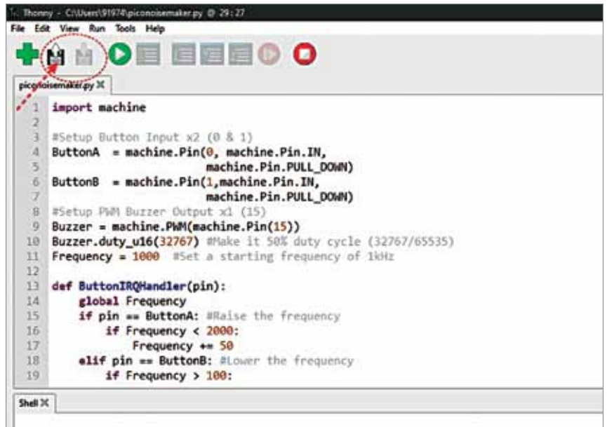
Fig. 4: Thonny editor window
