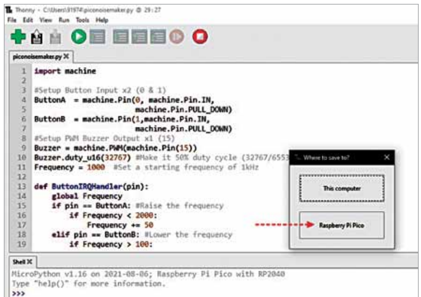
Fig. 5: Saving the Python code
