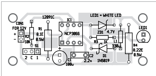
Fig. 4: Component layout of the PCB
