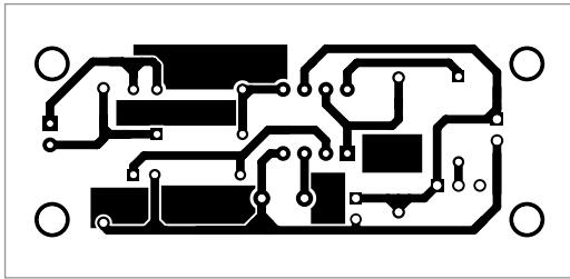
Fig. 3: Actual-size PCB layout of the circuit
