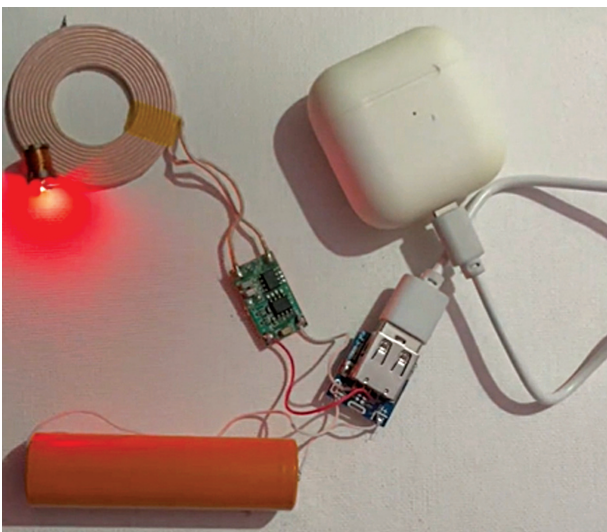
Fig. 2: Components used
