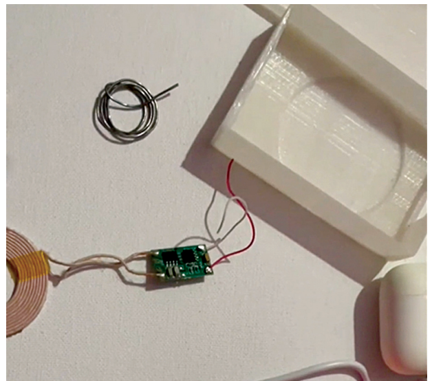
Fig. 4: 3D printed power bank case
