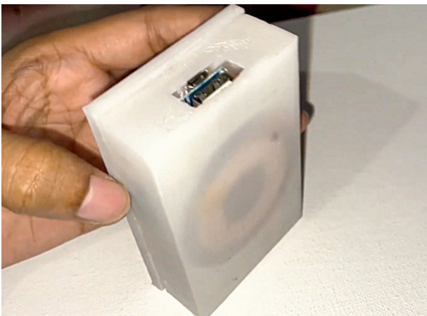
Fig. 1: MagSafe enabled wireless power bank
