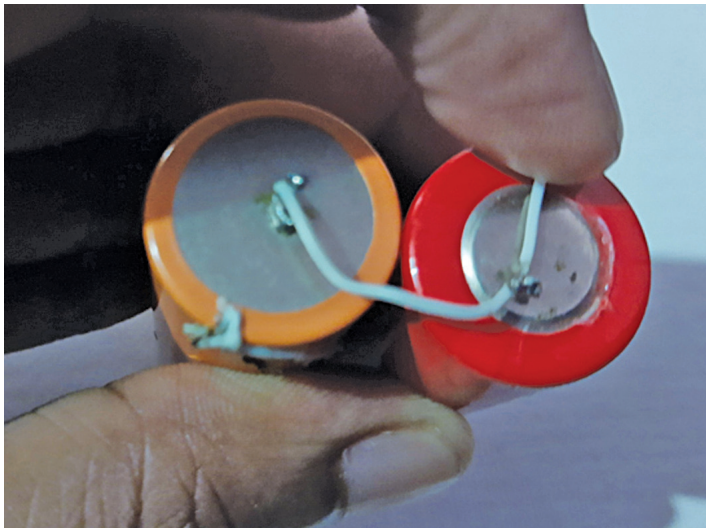
Fig. 6: Connecting the batteries in parallel
