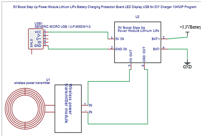
Fig. 5: Wireless power bank circuit
