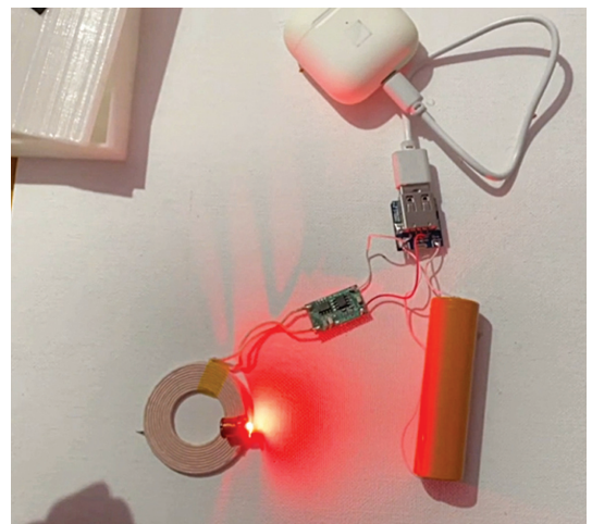
Fig. 9: Wireless transmitter charging module connected to the charger module
