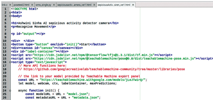
Fig. 6: JavaScript code
