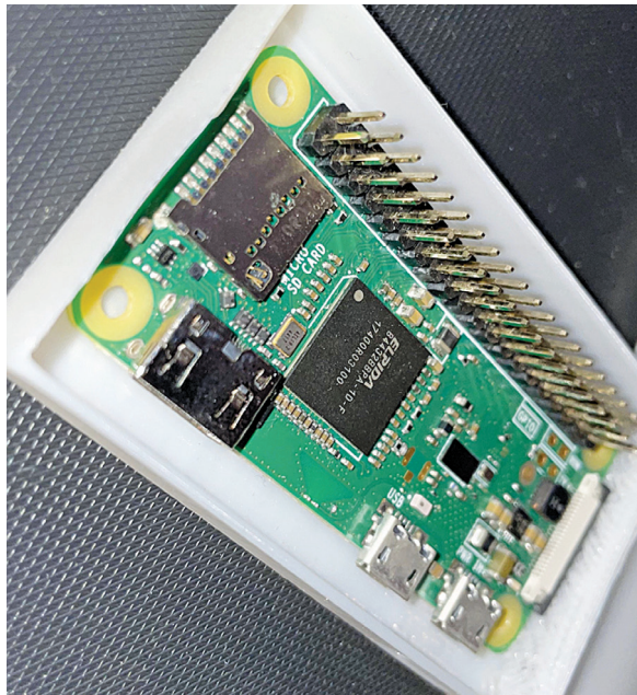
Fig. 14: E-ink header-to-header pins on Raspberry Pi
