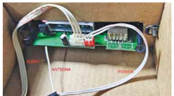
Fig. 11: Cables connected inside the cabinet
