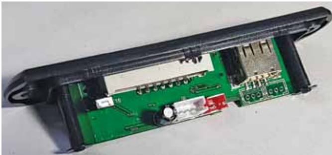
Fig. 5: Internal part of MP3 player module
