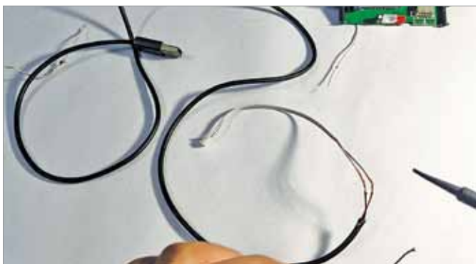
Fig. 7: Soldering the power cable to a type-A USB connector
