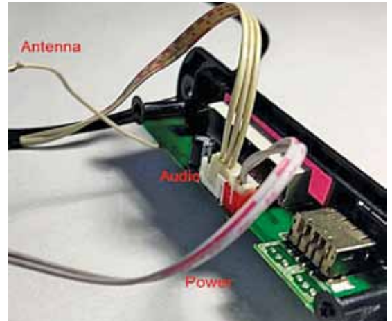
Fig. 9: Cable connections to MP3 player module
