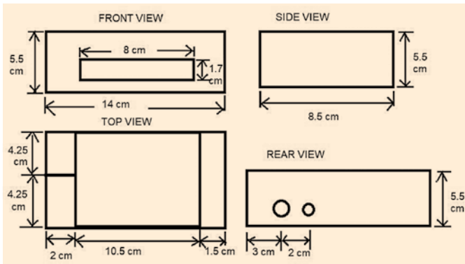
Fig. 4: Author's cabinet blueprint
