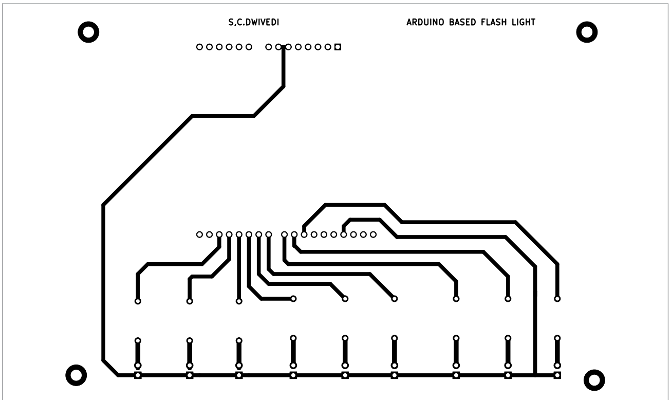
Fig. 4: Actual-size PCB layout for the circuit in Fig. 2
