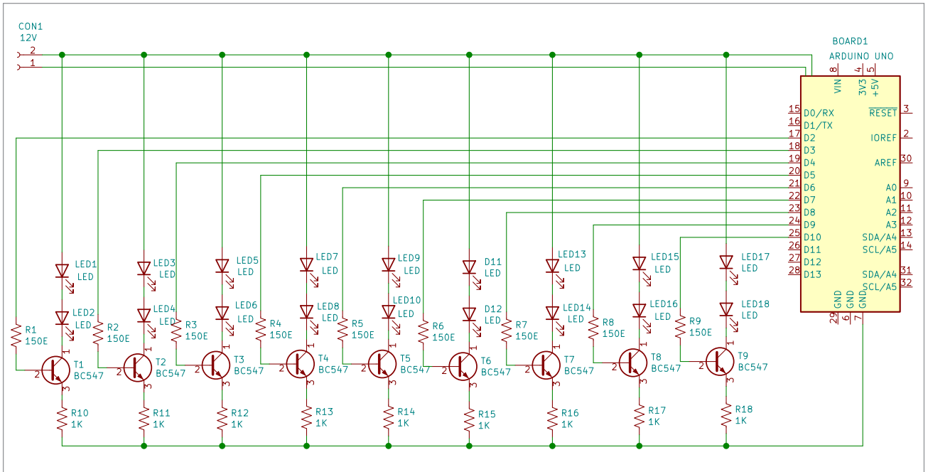
Fig. 3: Circuit diagram for 18 LEDs
