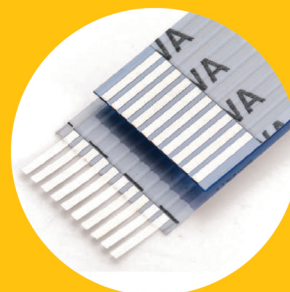
Open end Type for direct soldering
