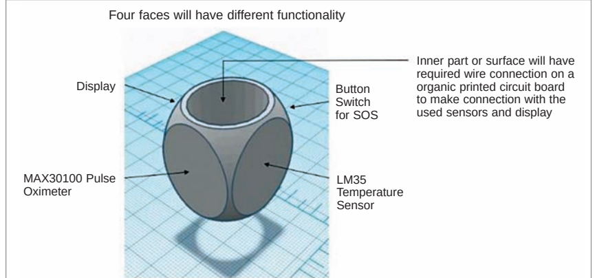
Fig. 3: Suggested placement of components in the ring
