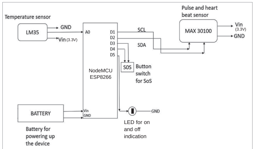
Fig. 4: Circuit diagram
