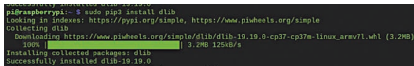
Fig. 4: Installing dlib
