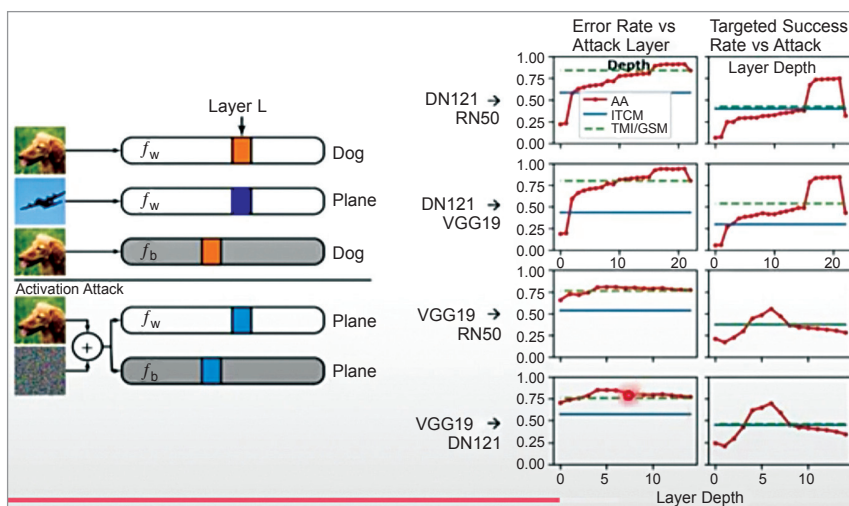
Fig. 13: Activation attack
