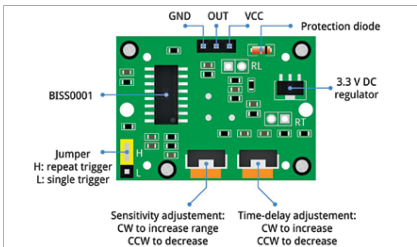
Fig. 3: Back side of the motion sensor
