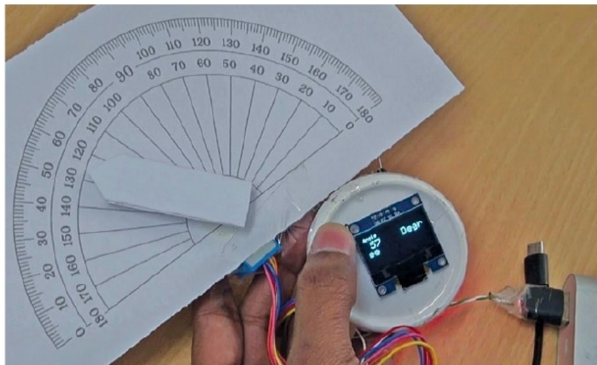
Fig. 9: Digital protractor calibration
