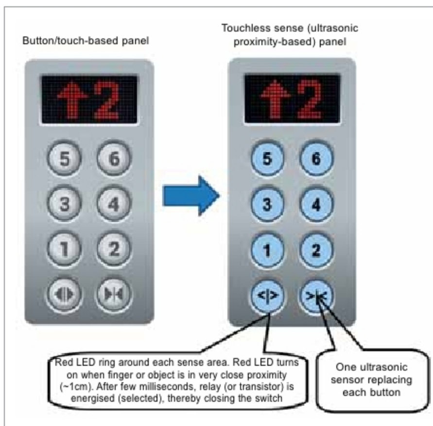
Fig. 3: Transformation from present button-based panel to touchless sense switching panel using ultrasonic sensors
