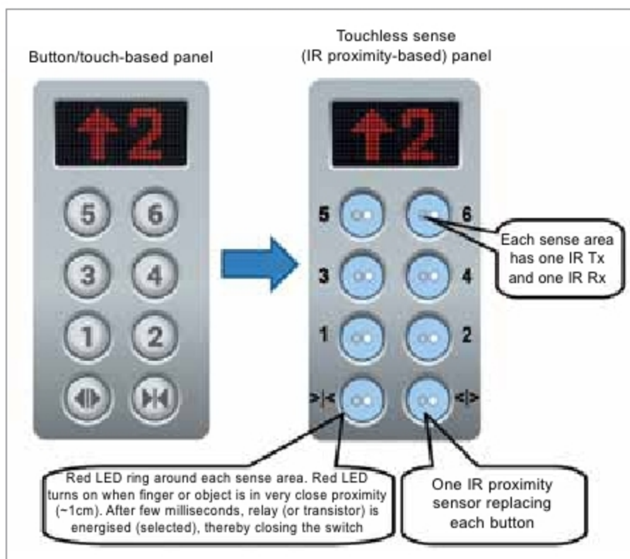
Fig. 4: Transformation from present button-based panel to touchless sense switching panel using infrared proximity sensors
