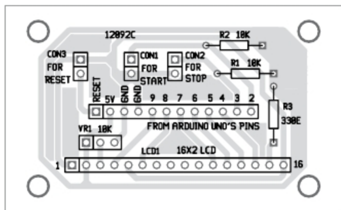
Fig. 4: Components layout of the PCB
