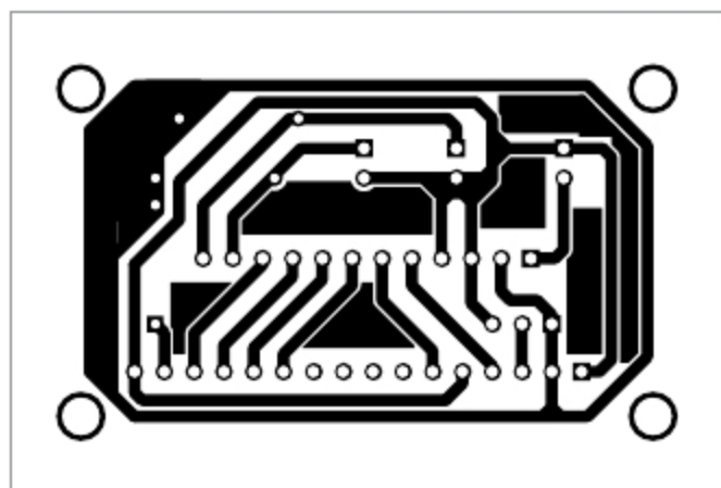
Fig. 3: Actual-size PCB layout for the timer kit
