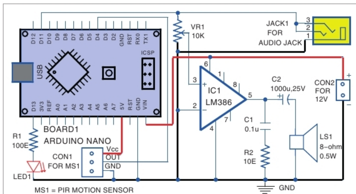
Fig. 3: Circuit diagram of motion sensor alarm
