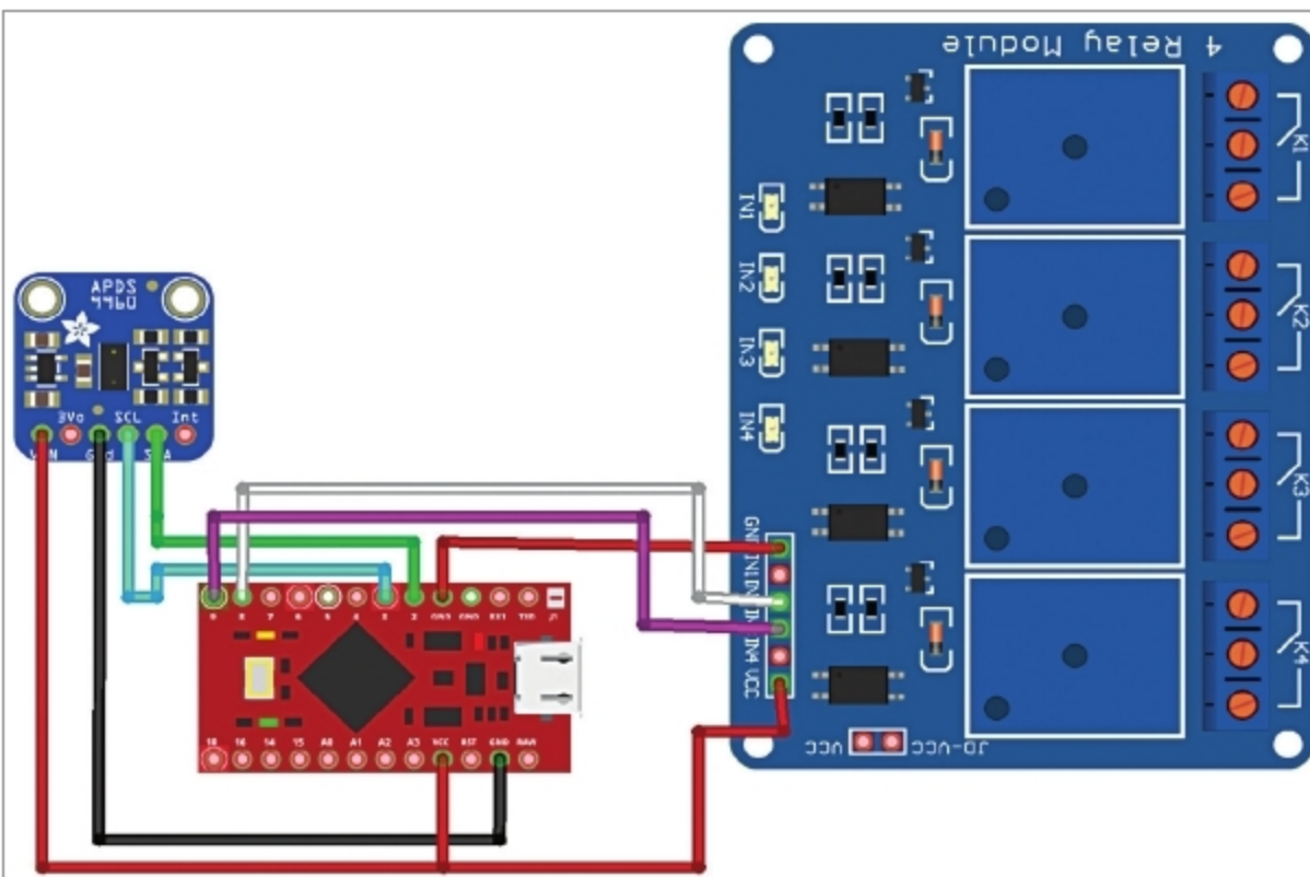
Fig. 6: Connection diagram
