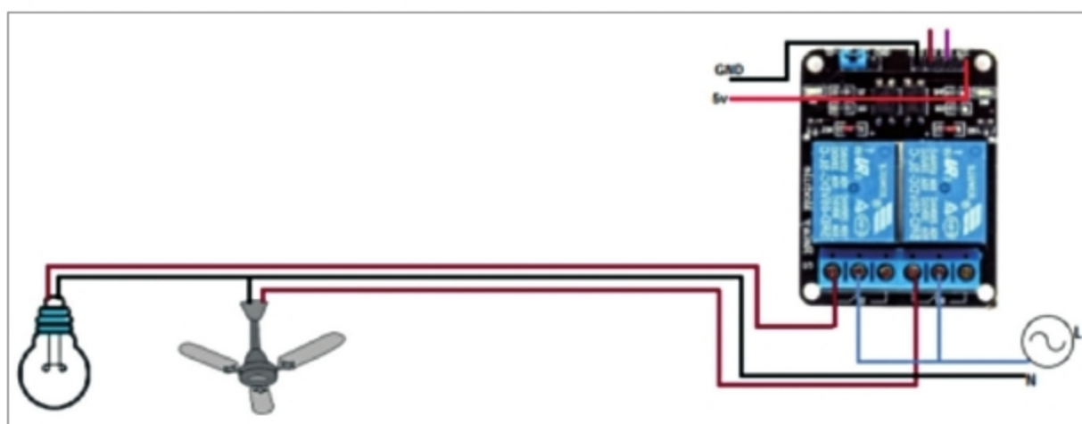
Fig. 7: Relay connections with bulb and fan
