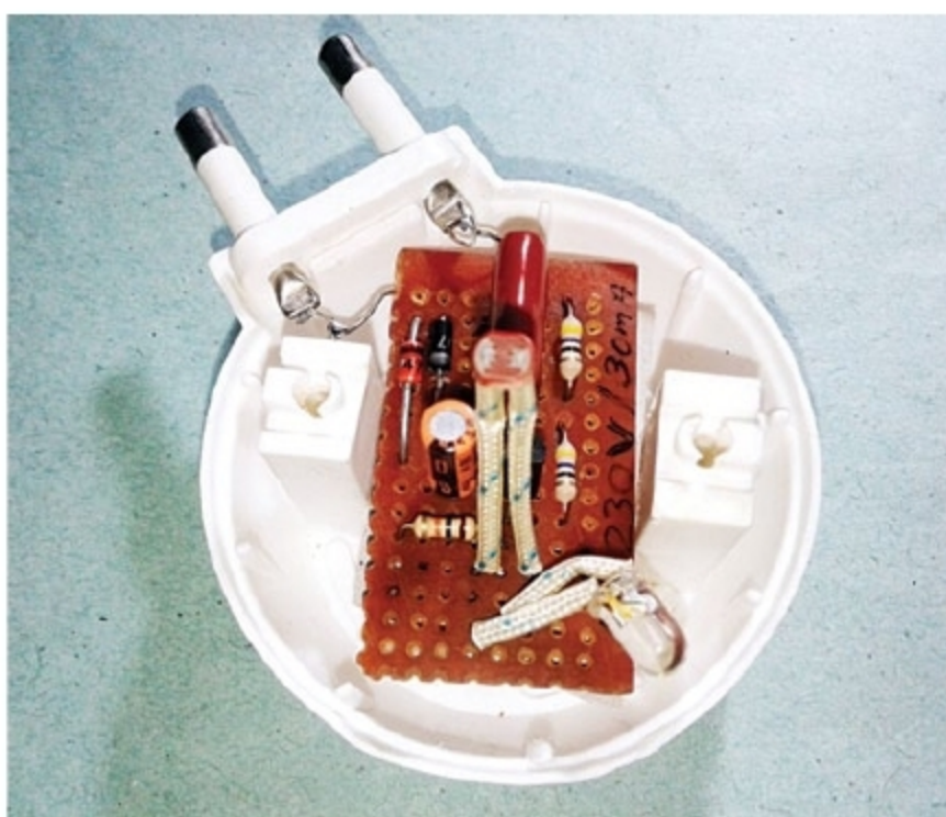
Fig. 6: Author's prototype
