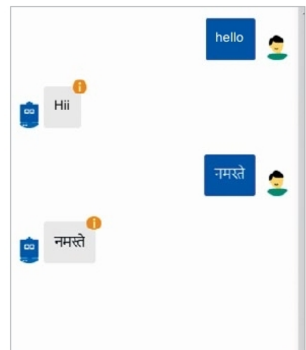
Fig. 15: Multi-language bot
