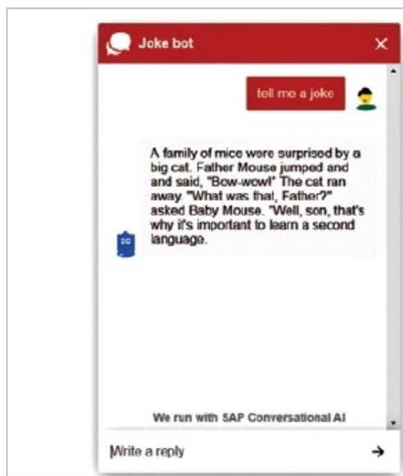
Fig. 13: Webchat deployed
