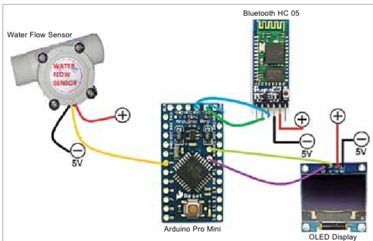
Fig. 12: Wiring diagram of smart water meter
