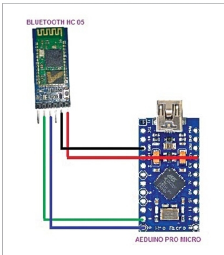
Fig. 8: Arduino Pro Micro connections (receiver)
