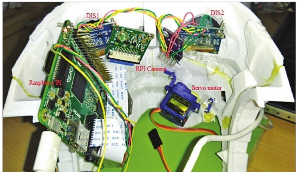
Fig. 3: Robot head assembly
