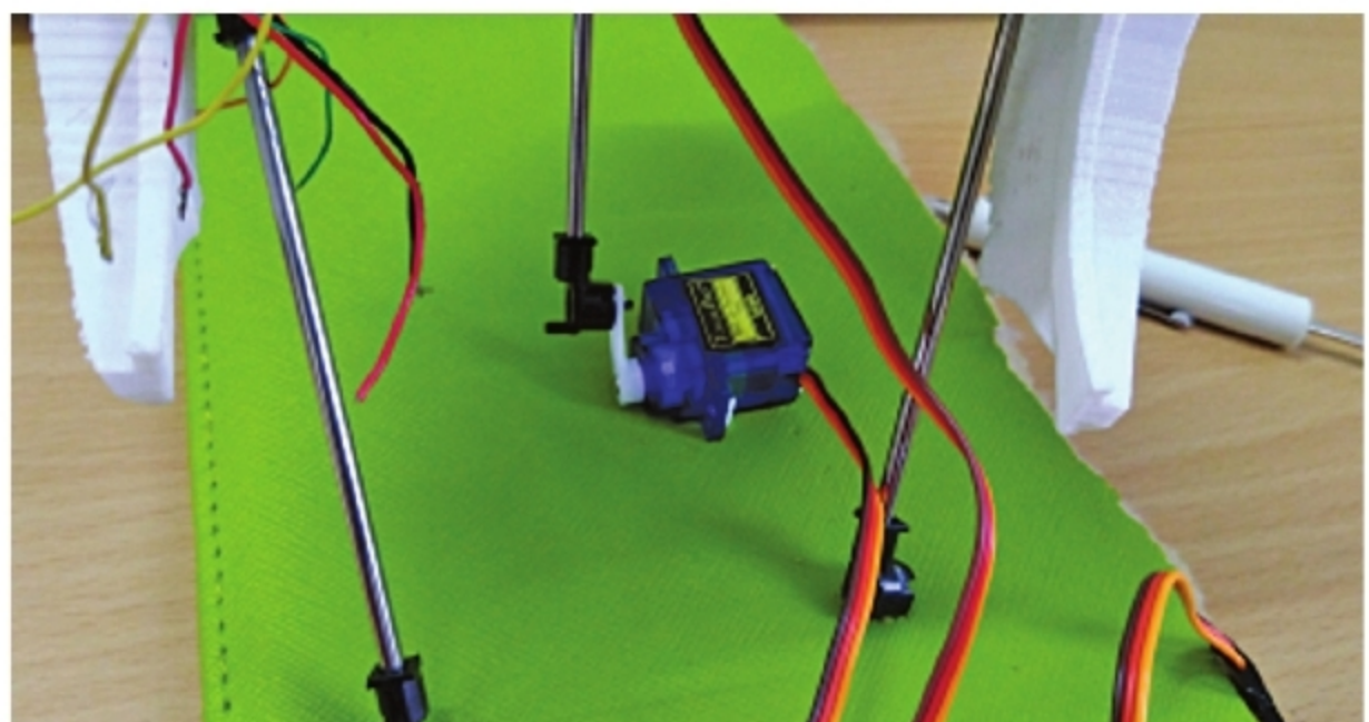
Fig. 5: Second servo motor placed on a cardboard base
