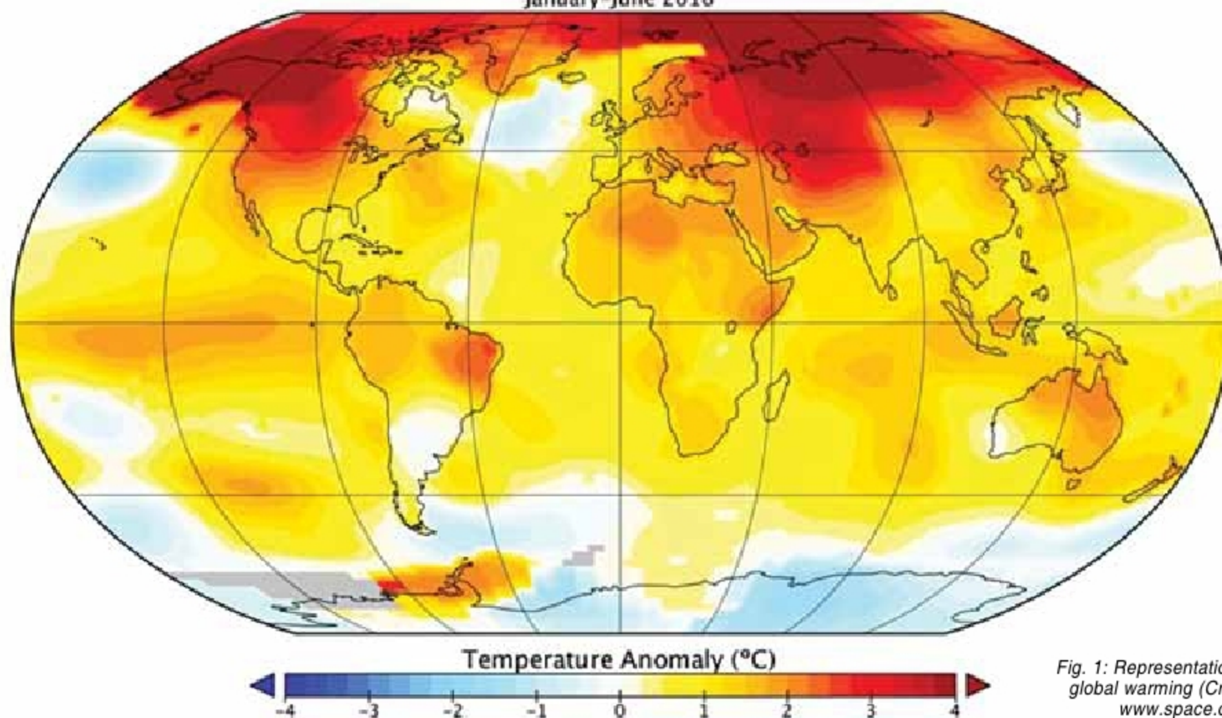
Global Mean Surface Temperature (GISS)
