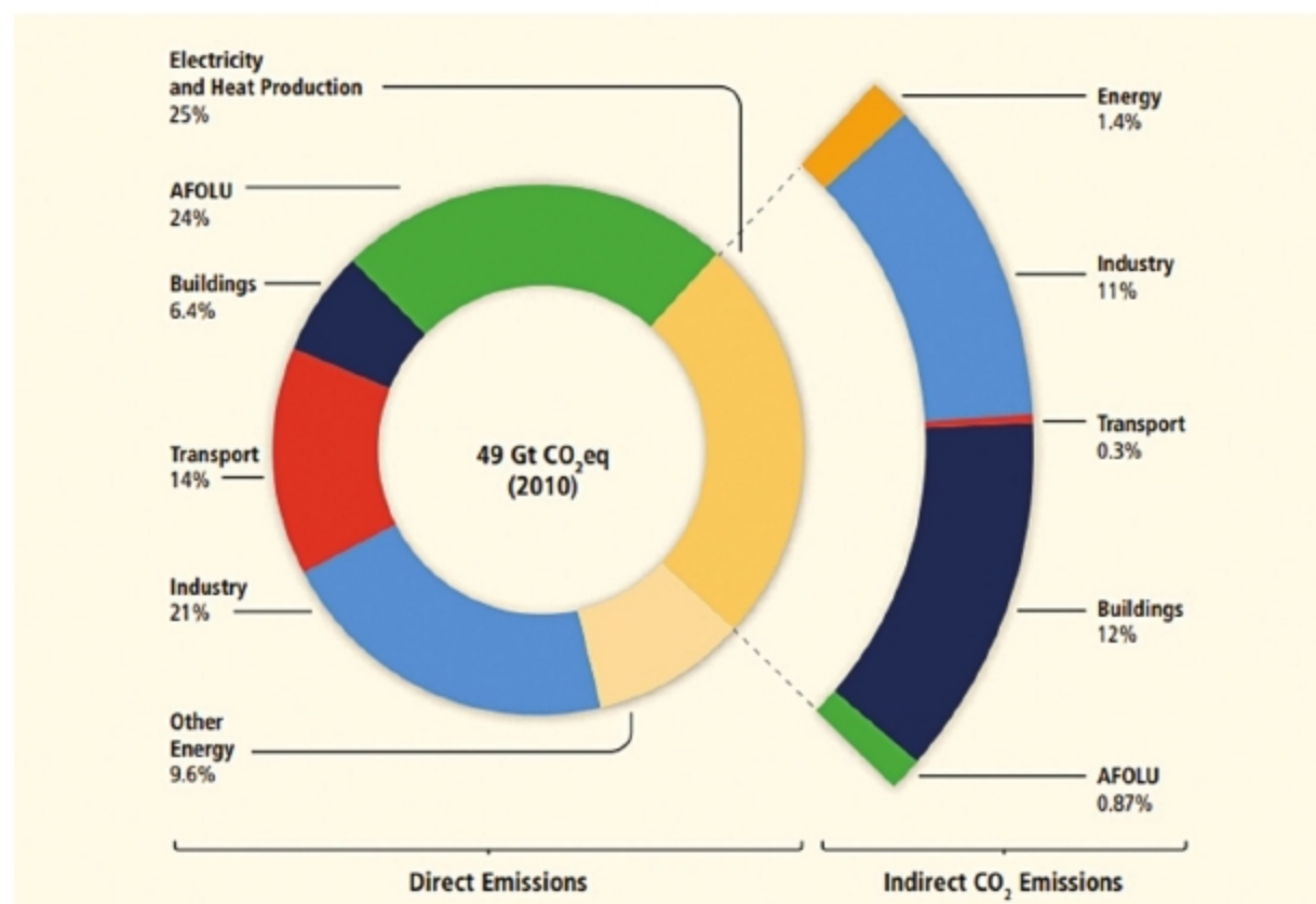
Fig. 2: The global greenhouse gas emission in 2010 (Credit: www.ipcc.ch)
