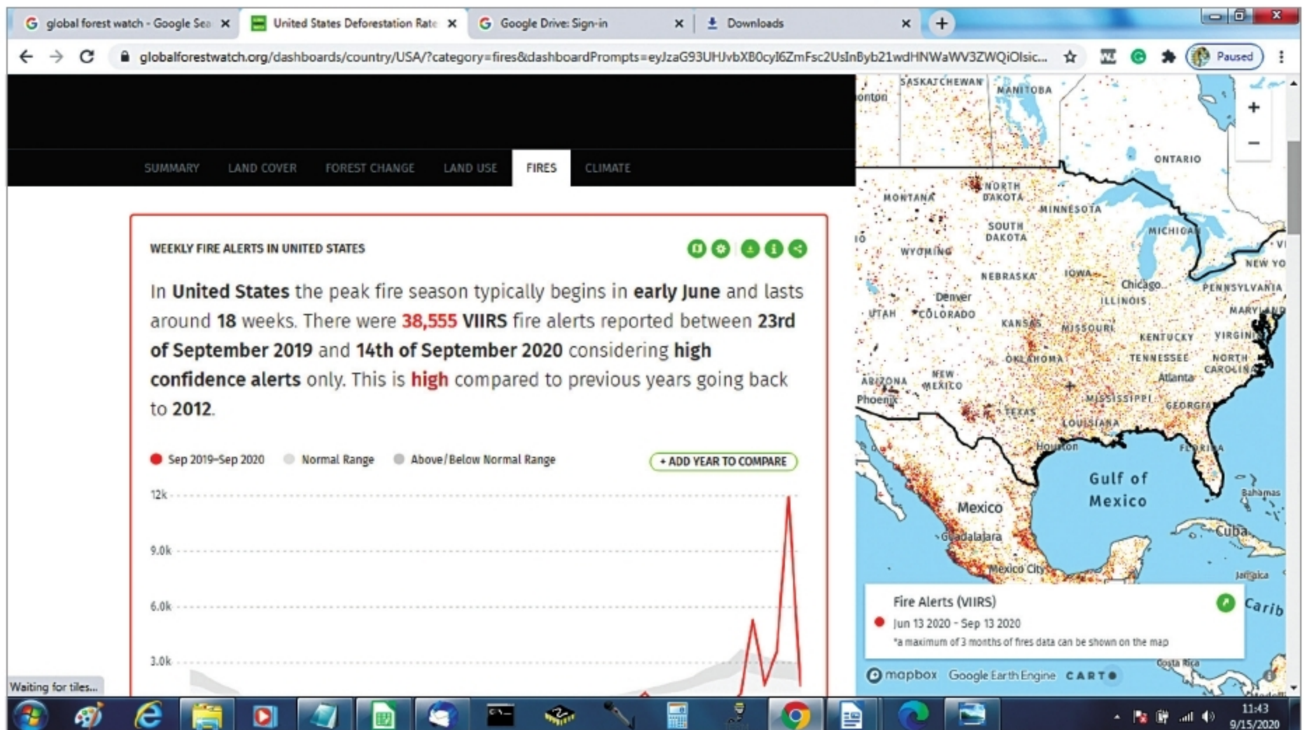
Fig. 3: Forest fire alerts in the United States in September (Credit: www.globalforestwatch.org )
