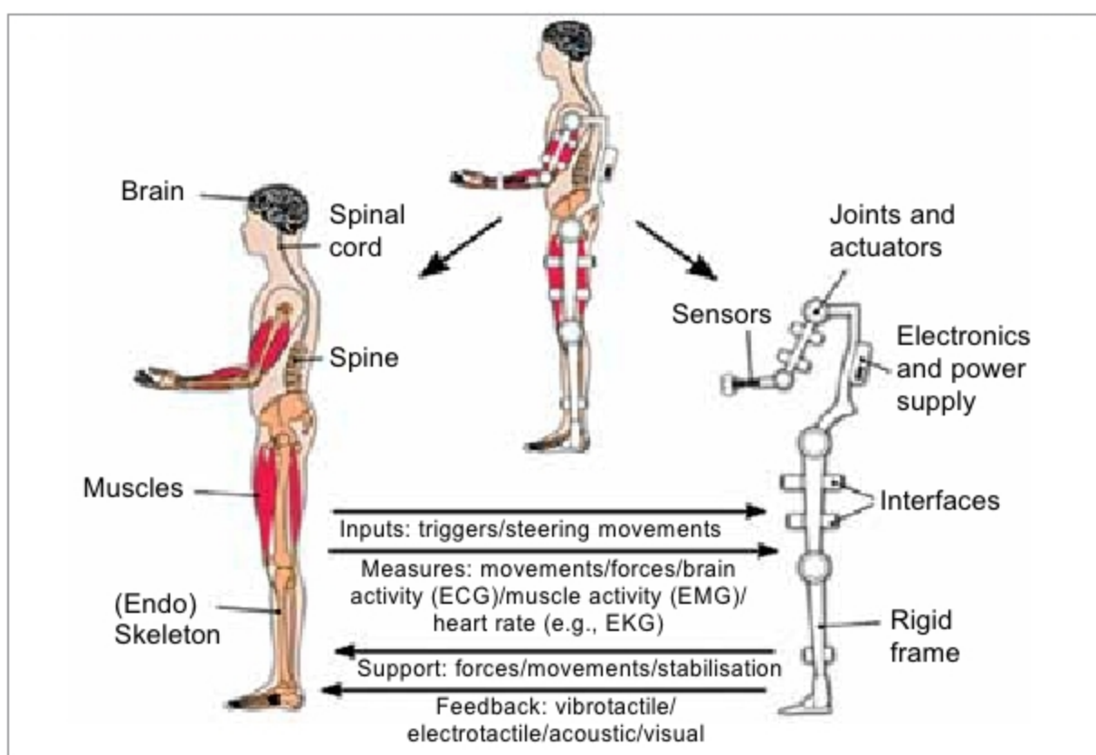
Fig. 11: Multi-layered exoskeleton-user interaction (Credit: eduexo.com/resources)
