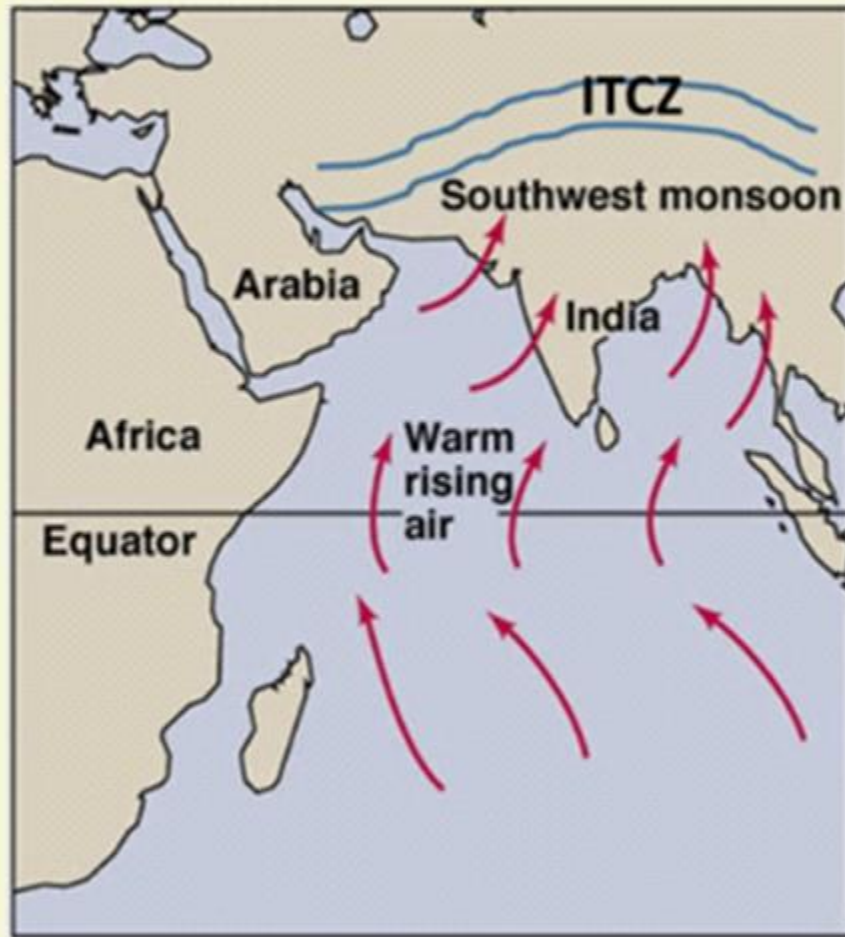
SOUTH-WEST MONSOON
