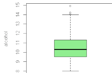
Boxplot of alcohol
