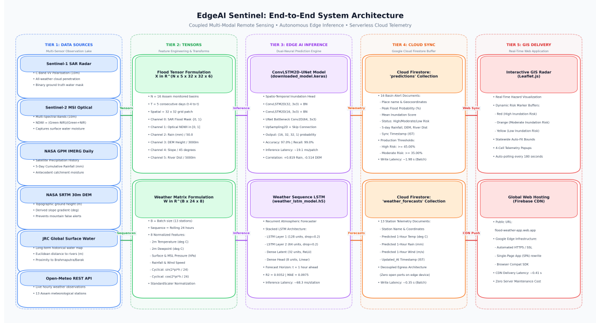
Figure 3.1: End-to-End Five-Tier System Architecture of the 5G-Enabled Edge AI Framework.
