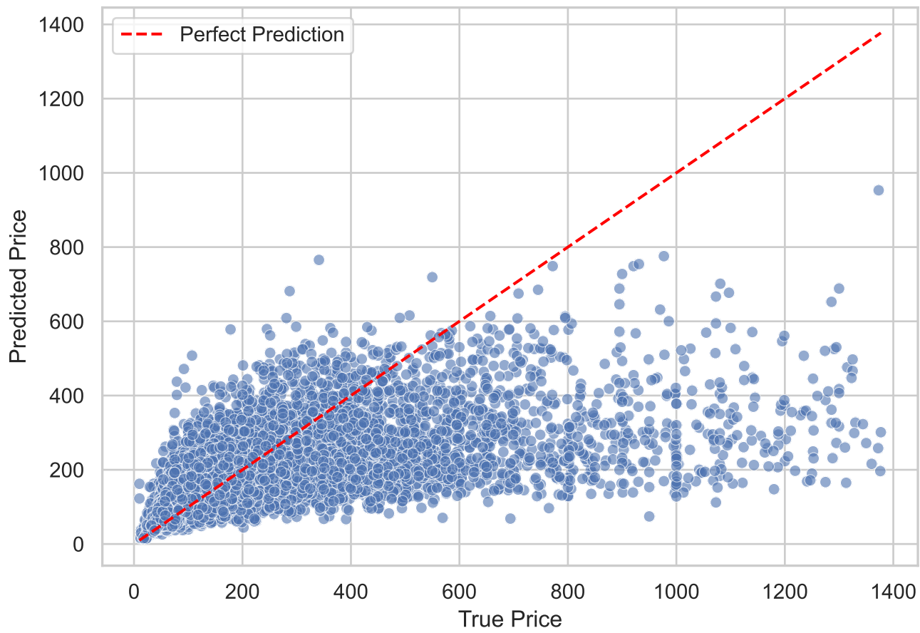
Medium Tier: Predicted vs True Prices
