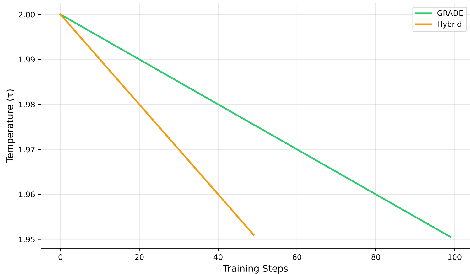
Gumbel-Softmax Temperature Annealing
