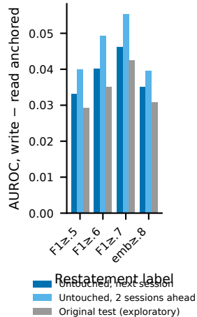
c Robust to label and horizon
